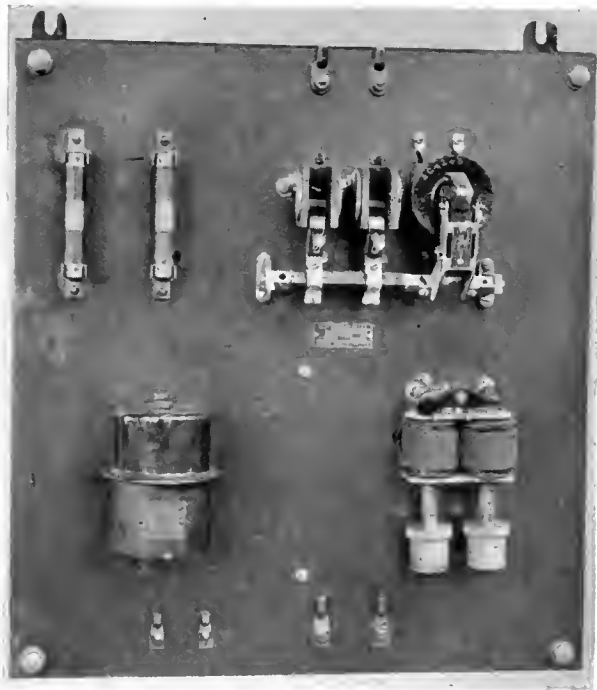
FIG. 2. TYPICAL SEMI-MAGNETIC CONTROL PANEL FOR HIGH RESISTANCE ROTOR SQUIRREL-CAGE MOTOR
